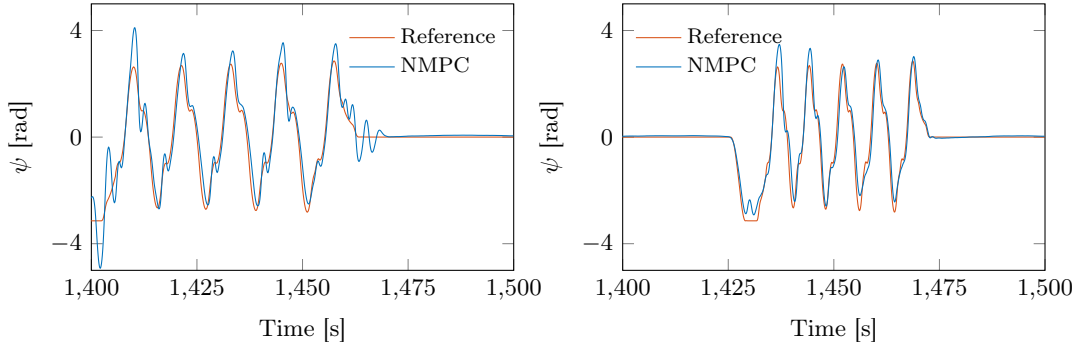
FIGURE 7.11: \psi performance considering nominal wind speed increase. Left: normal NMPC. Right: warping NMPC.
