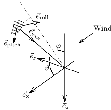
FIGURE 1.5: Kite model coordinate system [12].
