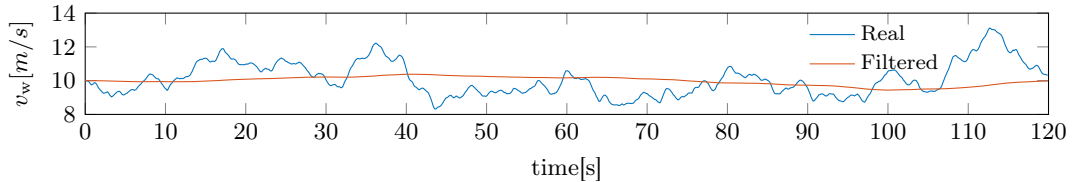
FIGURE 6.2: Wind profile for v_w^{(0)} = 10 m/s and a 10% turbulence.
