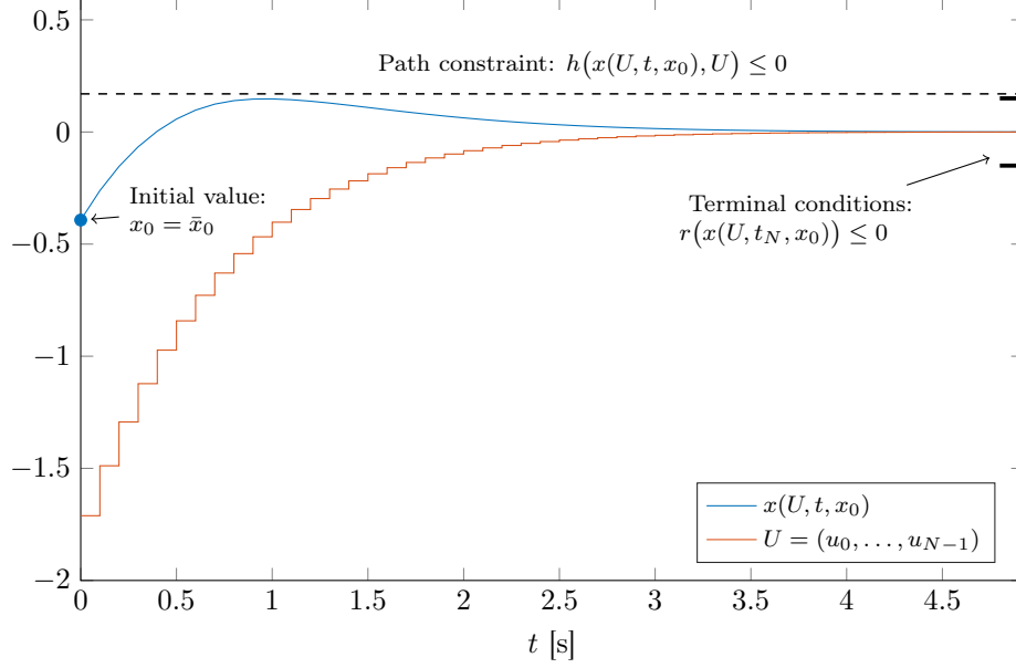
FIGURE 2.3: Single shooting OCP
